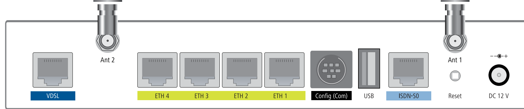
① VDSL ② Ant 2 ETH 4 ETH 3 ETH 2 ETH 1 Config (Com) USB ISDN-S0 Ant 1 Reset DC 12 V ⑦
