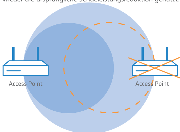
Abb. 7: Adaptive Transmission Power
